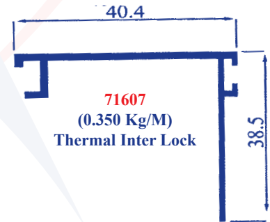
Sliding Shutter
