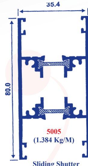
Sliding Shutter
