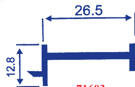
71603 (0.221 Kg/M) Adapter For Big Z
