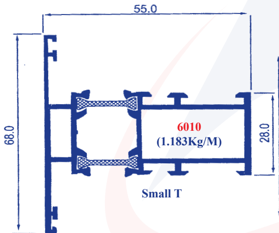
S/T Adapter
