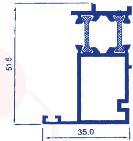
6009 (0.840 Kg/M) T Adapter (Small)
