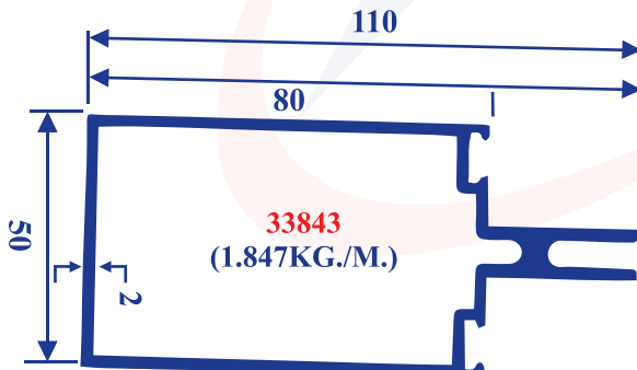
80 X 50 Curtain Wall with Nozle For ① Glass
