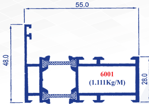
S/T Adapter
