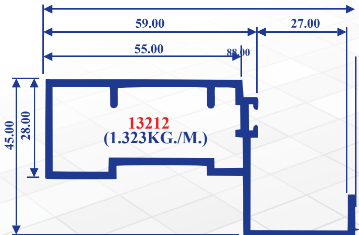
Curtain Wall Top (D/G)
