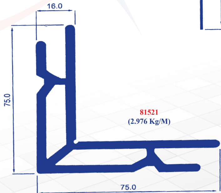
Thermal Inter Lock
