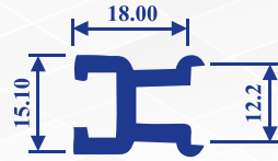
11472 (0.365K.G./M.) Curtain Wall Spacer
