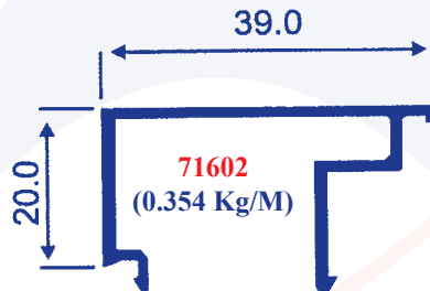
Single Glass Burclose
