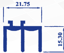
SC 231 Glass Sliding
