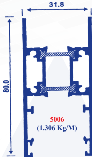
Sliding Shutter
