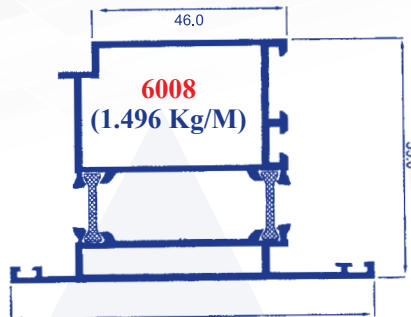
Shutter T Big
