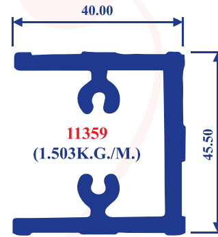
11359 (1.503K.G./M.) Curtain Wall Connector
