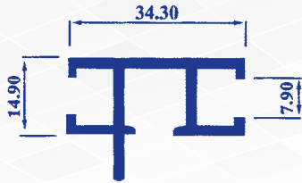
SC 230 SH. T. Section
