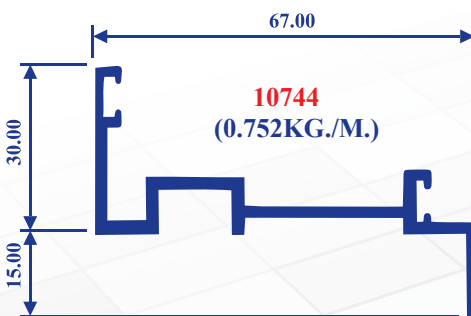
Curtain Wall Bottom (D/G)
